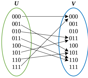
Figure 3: An example of injection and surjection in BCIEA.
